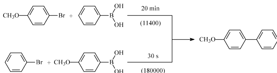
Scheme 1. Alternative paths for the formation of 4-methoxybiphenyl. Reaction conditions: aryl bromide (0.5 mmol), arylboronic acid (0.6 mmol), K 2 CO 3 (0.6 mmol), Pd(OAc) 2 (1 mol-%), EGME/H 2 O (3:1, 2 mL), T = 294 K. TOFs (in h -1 ) are reported in parenthesis.
