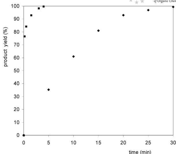
Figure 1. Comparison between the efficiency of Pd(OAc) 2 (■) and Pd(acac) 2 (◆) in the reaction between bromobenzene ( 1 ) (0.5 mmol) and 4-tolylboronic acid ( 2 ) (0.6 mmol) in the presence of K 2 CO 3 (0.6 mmol). Reaction conditions: EGME (1.5 mL), H 2 O (0.5 mL), T = 294 K.
