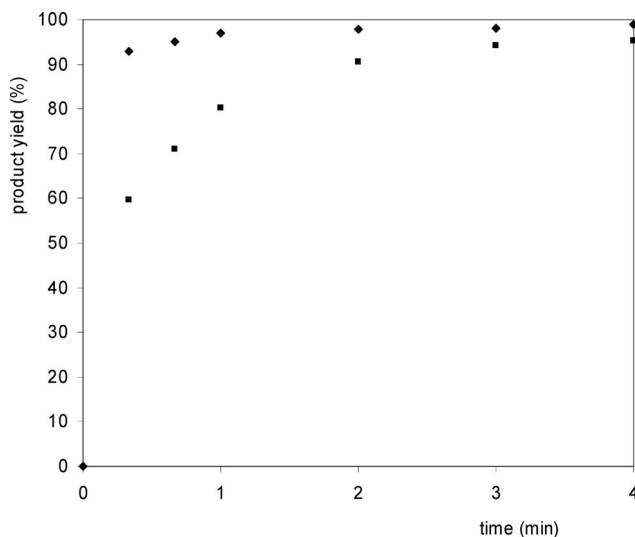
Figure 2. Yield of 4-methylbiphenyl ( 3 ) from bromobenzene ( 1 ) and 4-tolylboronic acid ( 2 ); (■) 0.5 mmol of TBAB added, (◆) without TBAB. Reaction conditions: 1 (0.5 mmol), 2 (0.6 mmol), K 2 CO 3 (0.6 mmol) EGME (1.5 mL), H 2 O (0.5 mL), T = 294 K.
